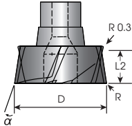
6 flutes D:16-25mm
