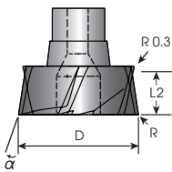
6 flutes D:16-25mm
