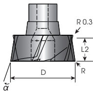
6 flutes D:16-25mm
