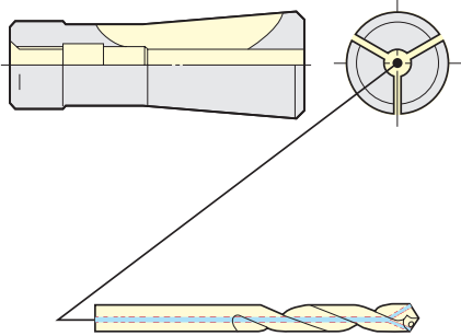
Cutting tool with internal cooling
