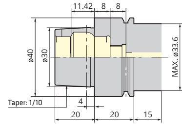
HSK40E (DIN69893-5)
