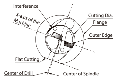
Fig.8 Excessive Offset (For Smaller Hole Diameter)
