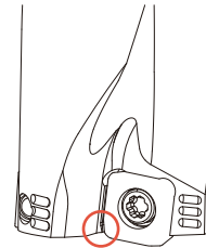
Fig. 11: Insert breakage near the centre of the drill.
